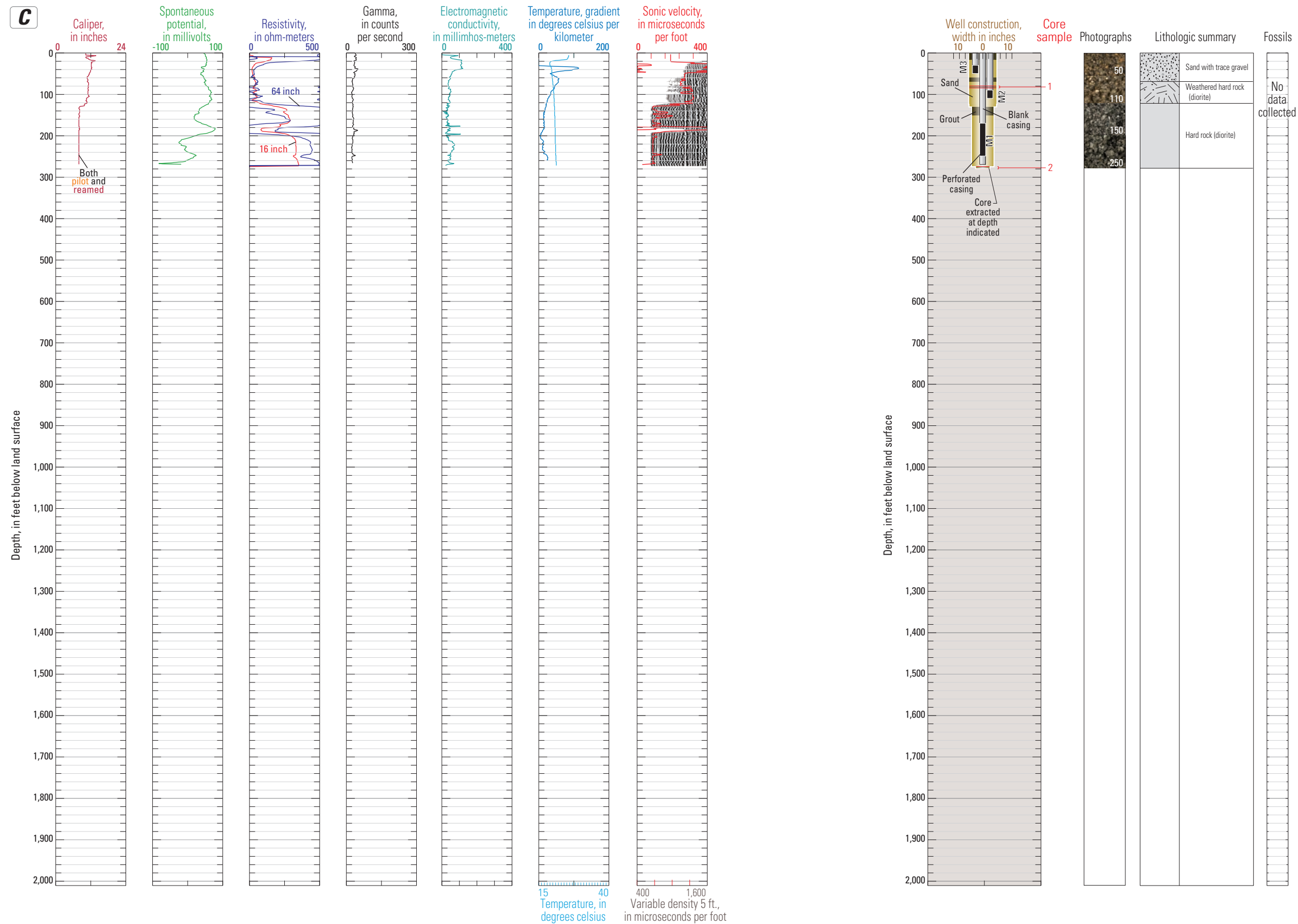
Figure 19C. Well-construction diagrams, generalized lithologic descriptions, and geophysical-log data for caliper, spontaneous potential, resistivity, natural gamma, electromagnetic conductivity, temperature, and sonic logs collected from 16 USGS multiple-depth, monitoring-well sites in San Diego County, California, 1995, 2003–2017: (A) SDCD; (B) SDSY; (C) SDLH ; (D) SDAQ; (E) SDCP; (F) SDBP; (G) SDHF; (H) SDEP; (I) SDNB; (J) SDSW; (K) SDMC; (L) SDLD; (M) SDCC; (N) SDOR; (O) SDOT; and (P) SDBW.—Continued.
